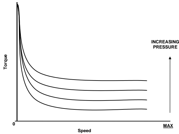
Figure 4.7 Progressive Cavity Pump Speed Torque Relation
