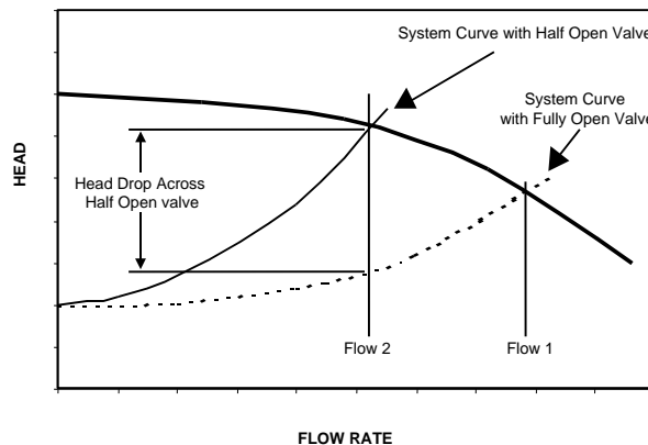
Figure 3.8 Control of pump flow by changing system resistance using a valve.
