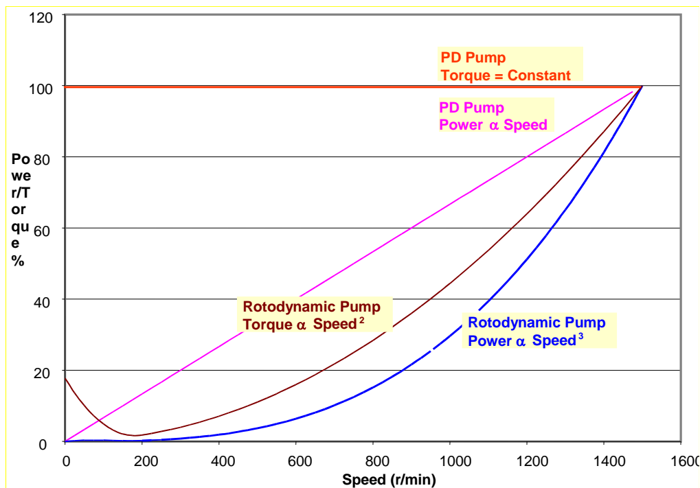
Figure 6.1 Power and torque vs. speed
