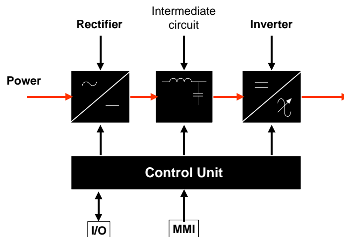
Figure 6.2 Basic Elements of frequency converter
