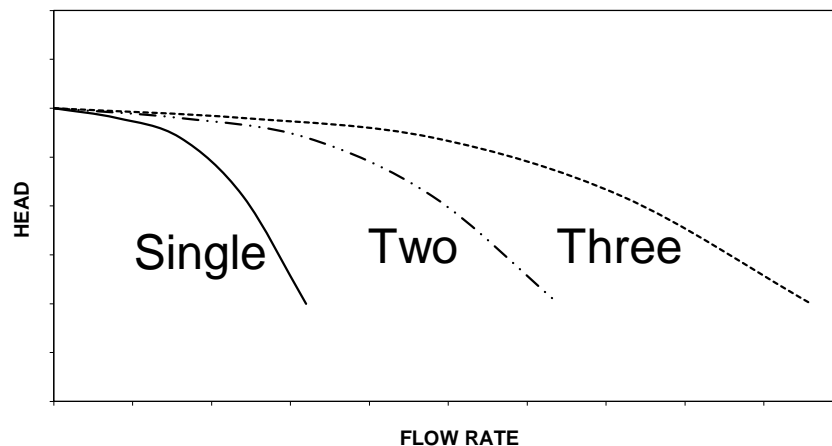
Figure 3.6 Typical head-flow curves for pumps in parallel
