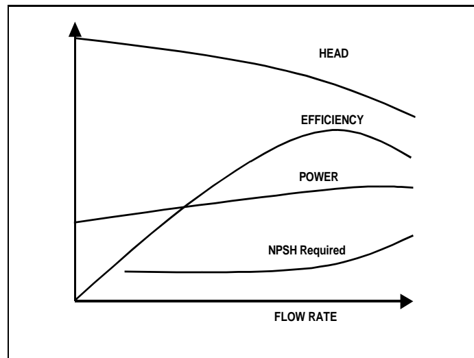
Figure 3.1: Example of Pump performance curves
