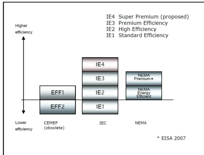
Figure 5.1 Rough relationship between the IE and EFF and NEMA levels
