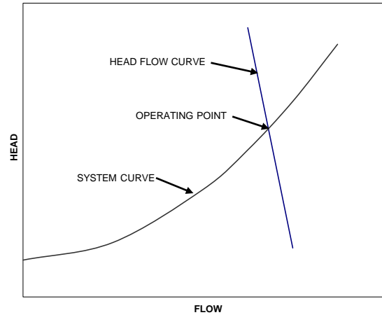
Figure 2.9 P.D. pump with system curve
