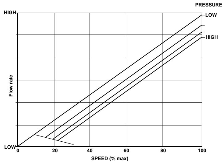
Figure 4.5 Speed/Flow Rate
