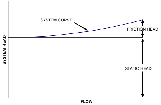
Figure 2.4 System with high static head
