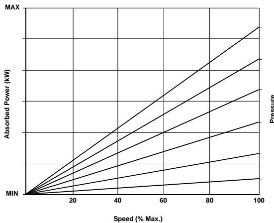
Figure 4.8 Rotary Pump Power Curve
