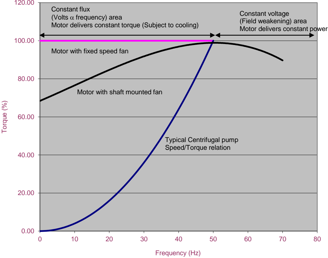
Figure 8.1 Typical Isothermal Loadability Curves
