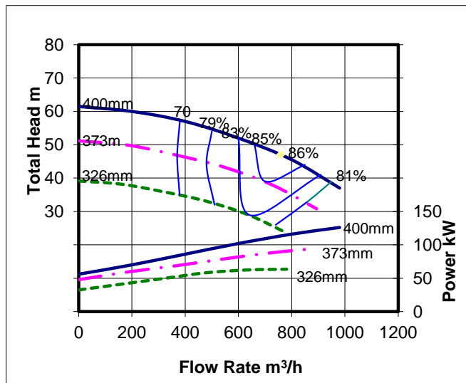
Figure 3.3 Example of impeller diameter reduction on rotodynamic pump performance.
