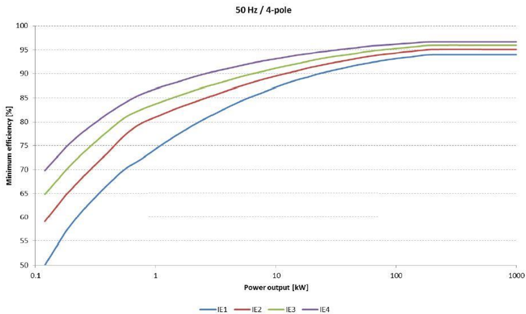
Figure 5.4 IE class for 50 Hz 4-pole motors according to IEC 60034-30-1:2014
