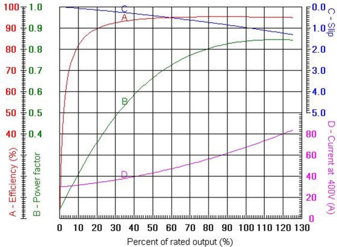
Figure 5.5 Typical relationship between efficiency, power factor and rated output
